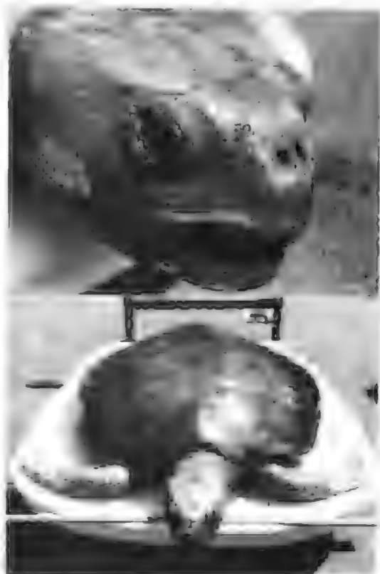
Fig. 3. Natator depressa lectotype (MCZ 4473). A. Head showing distinct preocular scute (po). B. Whole mount showing flattened carapace with reflexed lateral marginal rim and indistinct scutes. Ruler = 1 m.
